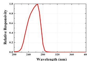
Fig. 2 Responsivity Curve
